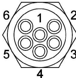
Figure A-8: MCBH6M Bulkhead, Male Face View
