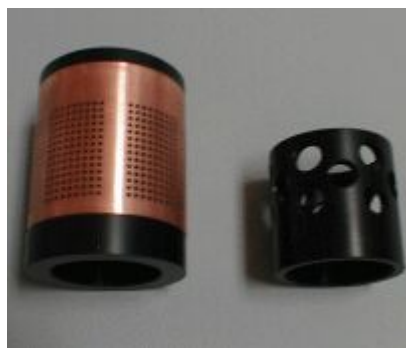
Figure A-13: Probe Guards
