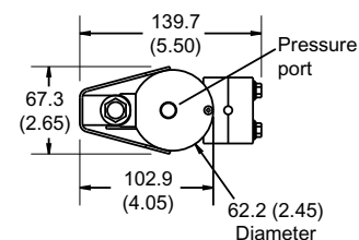
Dimensions in mm (inches)
